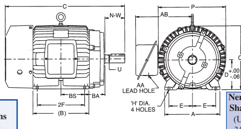
Typical Rigid Base Motor
