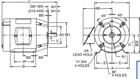
Typical C-Face Motor
