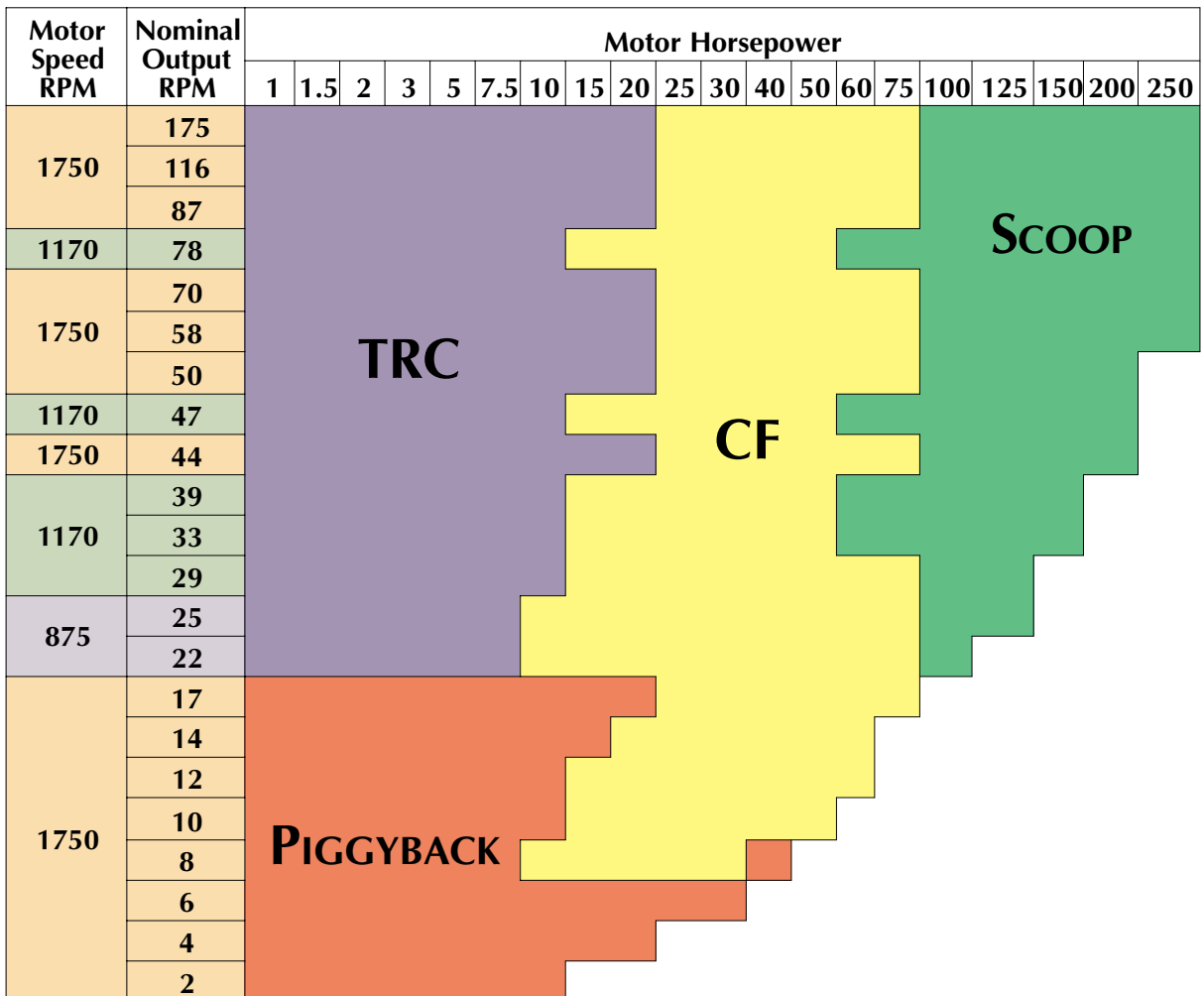
DORRIS DIRECT DRIVE REDUCER SELECTION CHART: CLASS 2 (NORMAL DUTY) SERVICE
